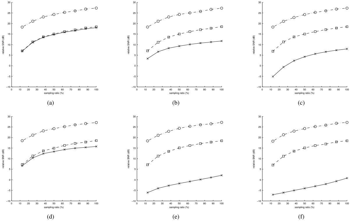
Fig. 4. Reconstruction performance versus under-sampling ratio: ‘o’ oracle reconstruction, ‘□’ Algorithm 2 and ‘x’ oracle post-processing autofocus. Quadratic: (a) \gamma = 0.1 (b) \gamma = 1 (c) \gamma = 10 . Random: (d) \gamma = 0.1 (e) \gamma = 1 (f) \gamma = 10 .
