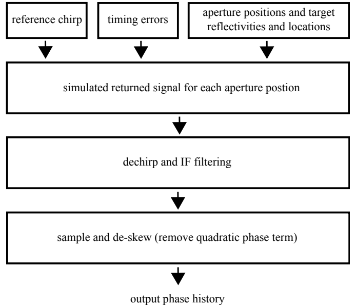
Fig. 5. block diagram for generating a simulated phase history
